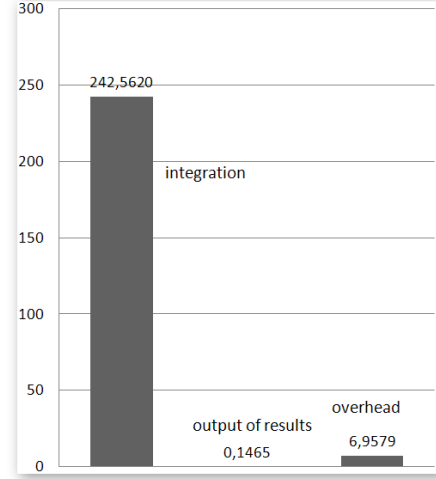
Figure 3: Workload in global steps
