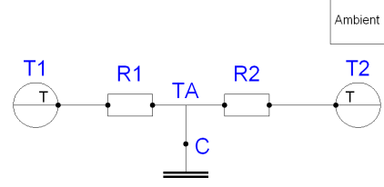
Figure 12: Optimized thermal circuit
