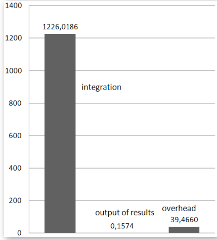
Figure 10: Workload in global steps
