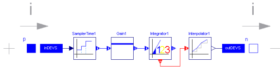
Figure 10: The internal structure of the ModelicaDEVS capacitor.
